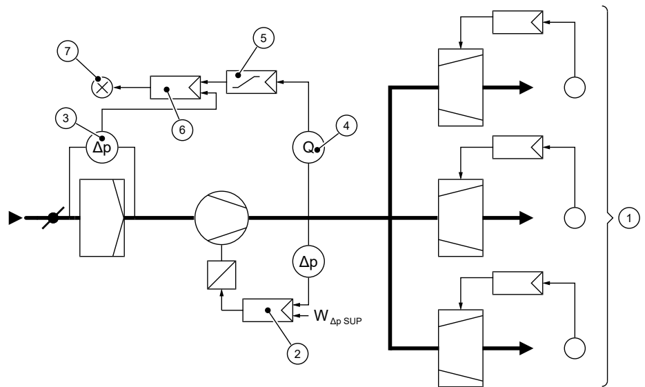
Fig. 119: Principal schema filter monitoring
