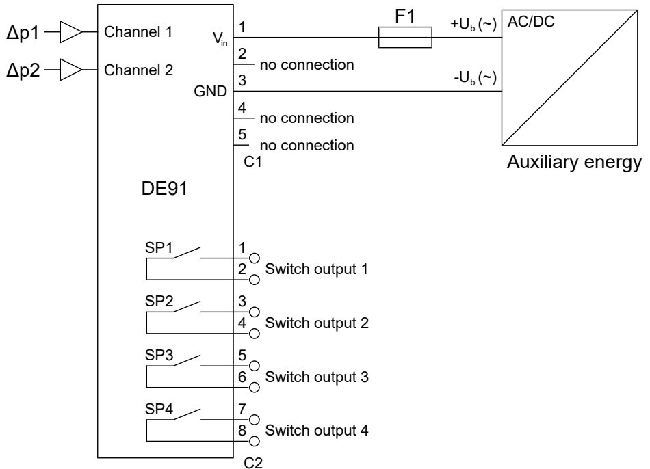
Fig. 12: 2-channel version (without analogue output)
