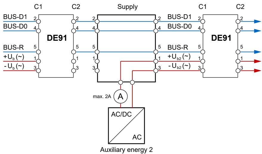
Fig. 27: Intermediate supply
