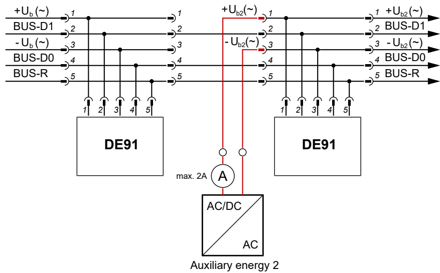
Fig. 34: Intermediate supply
