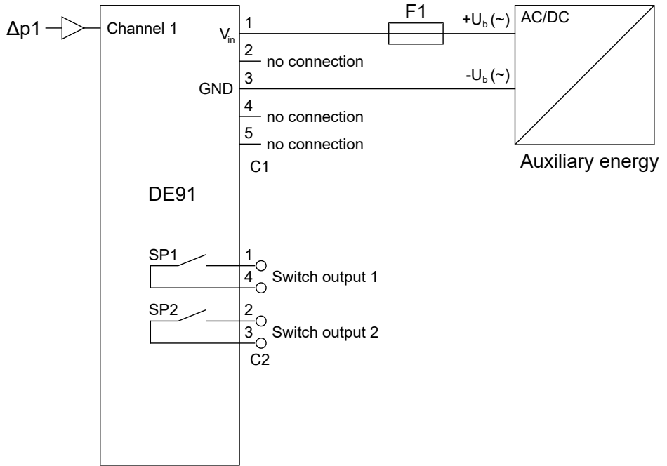
Fig. 11: 1-channel version (without analogue output)
