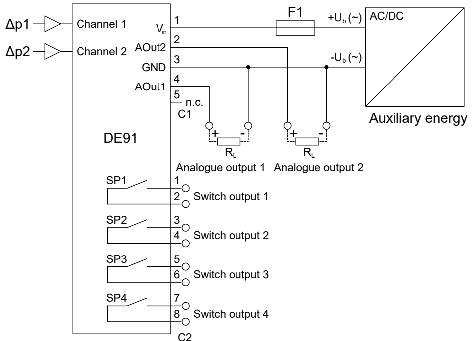
Fig. 18: 2-channel version (with analogue output)
