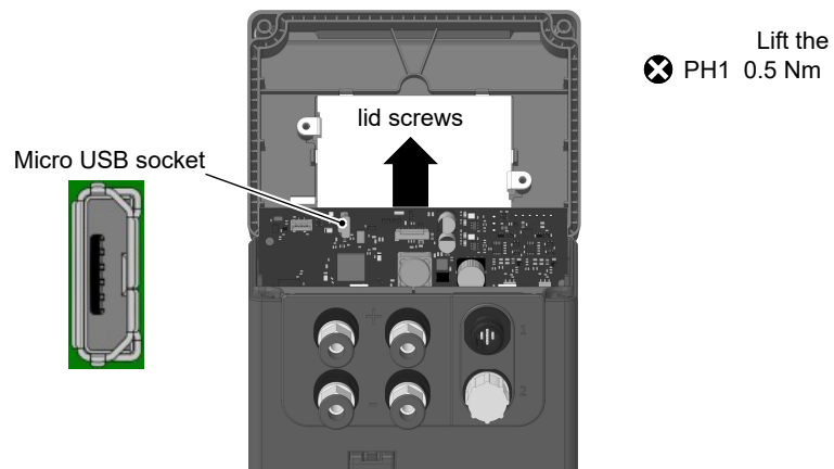
Fig. 148: USB port (example)
