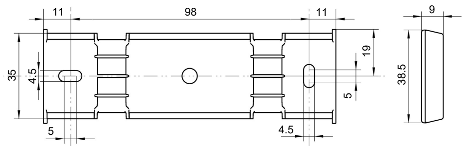
Fig. 152: Mounting rail
