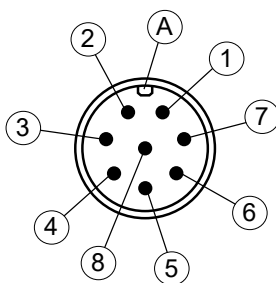
Fig. 22: M12 plug 8-pin
