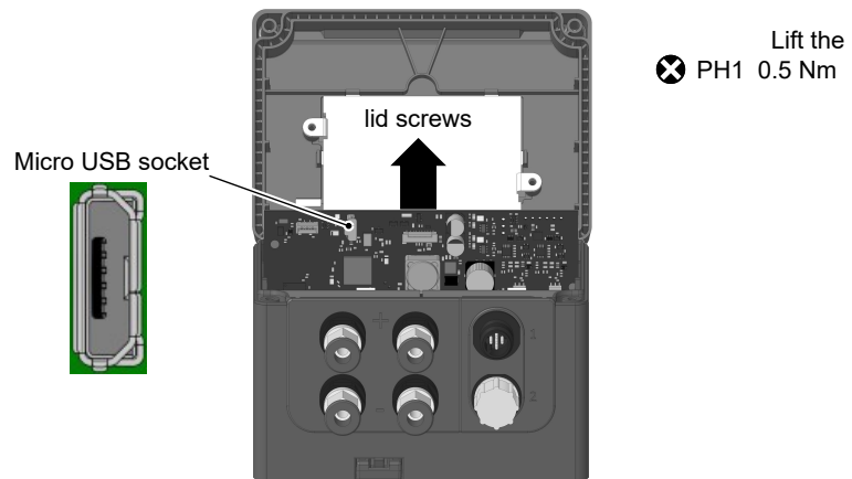
Fig. 40: USB port (example)
