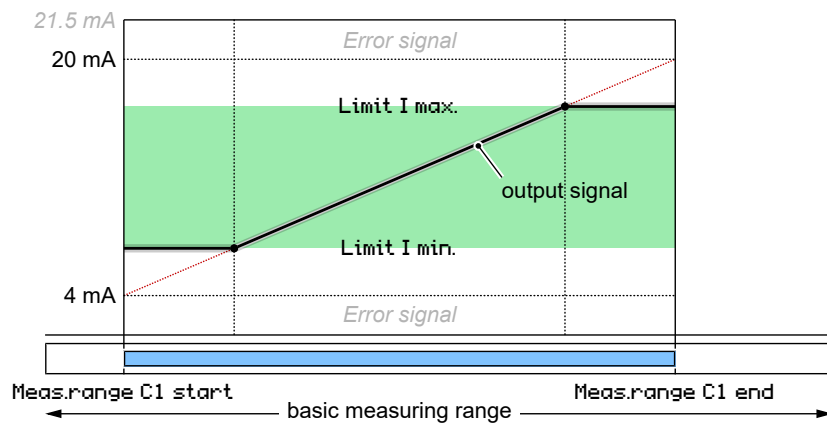
Fig. 126: Limitation of the output signal
