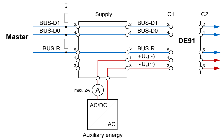
Fig. 26: Main supply
