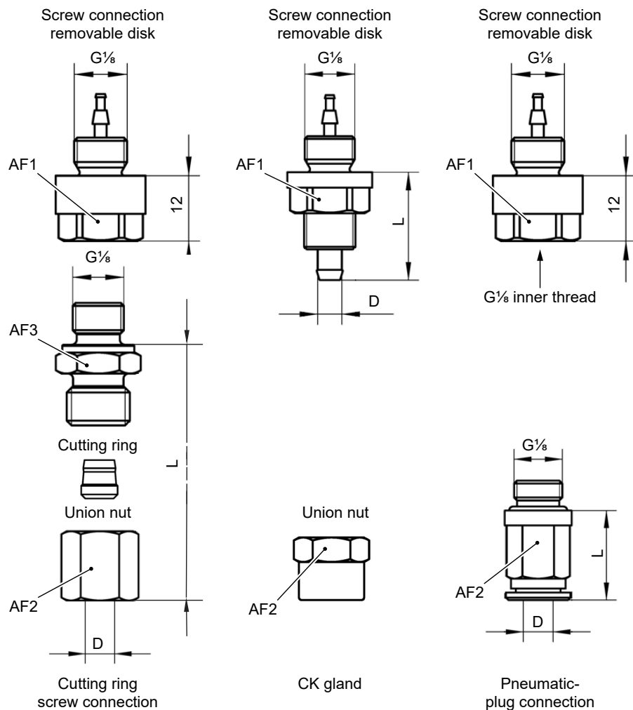
Fig. 153: Process connection Options
