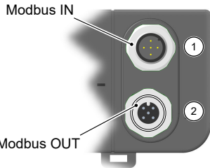
Fig. 23: Modbus replacement plate
