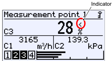
Fig. 117: Zero point window degree of contamination
