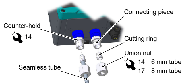
Fig. 9: Counter-hold for cutting ring screw connections
