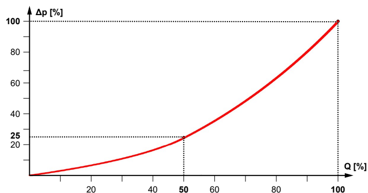
Fig. 120: General filter characteristic
