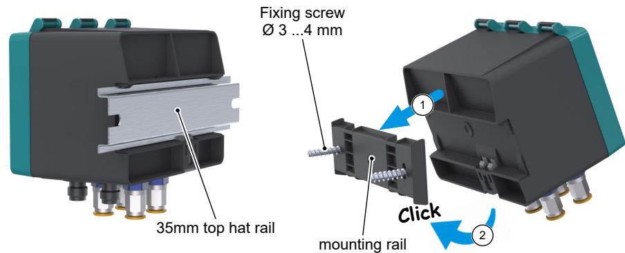
Fig. 6: Assembly
