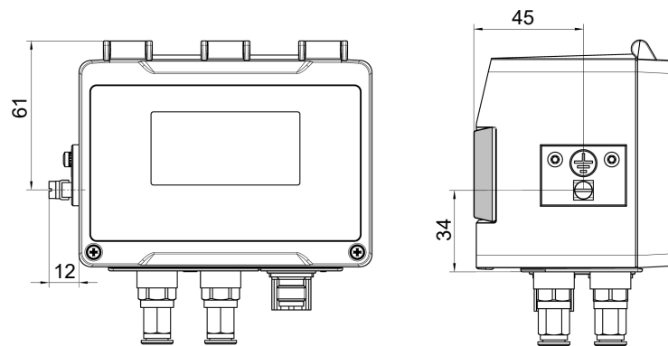
Fig. 151: Dimension drawing ATEX
