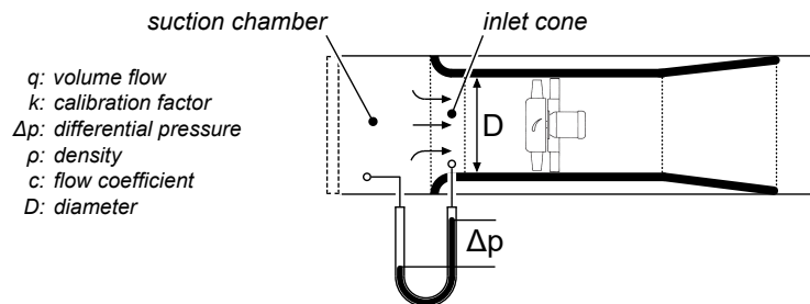
Fig. 91: Volumetric flow measurement Manufacturer's formulas
