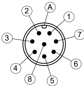
Fig. 36: 8-pin M12 connector
