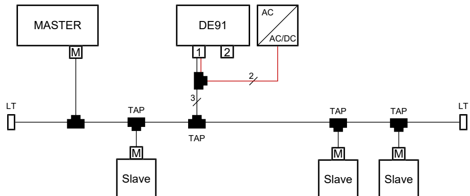
Fig. 32: Modbus connection
