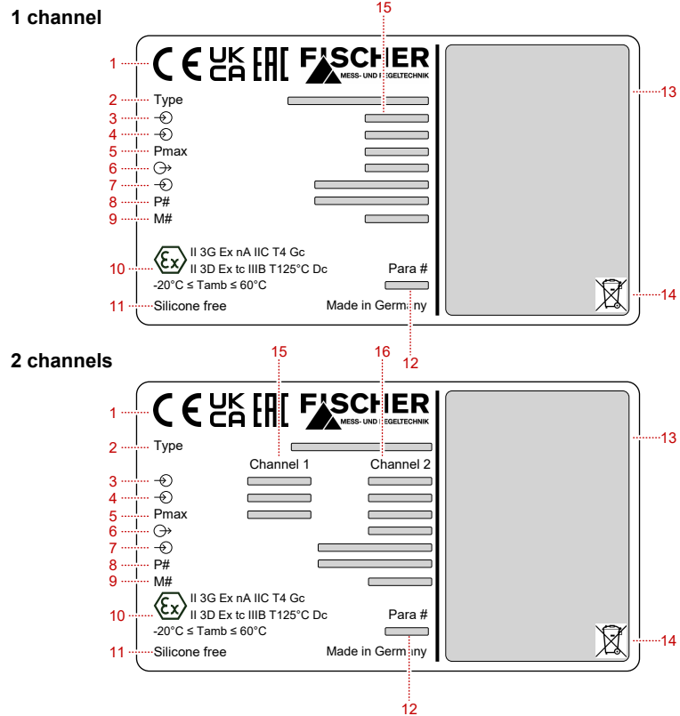
Fig. 5: Type plate
