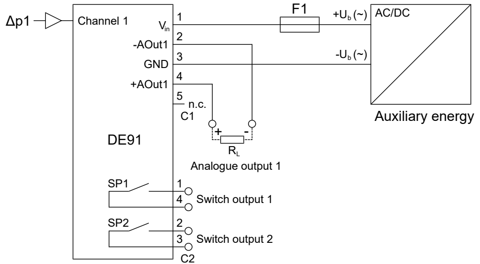
Fig. 17: 1-channel version (with analogue output)
