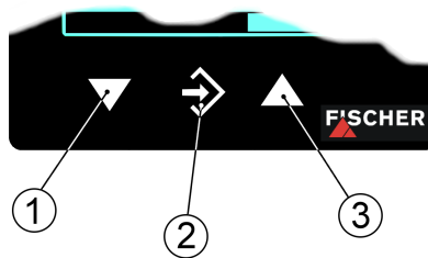
Abb. 14: Bedientasten [LC-Anzeige]
