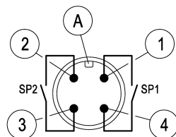
Abb. 23: M12 Stecker 4pol
